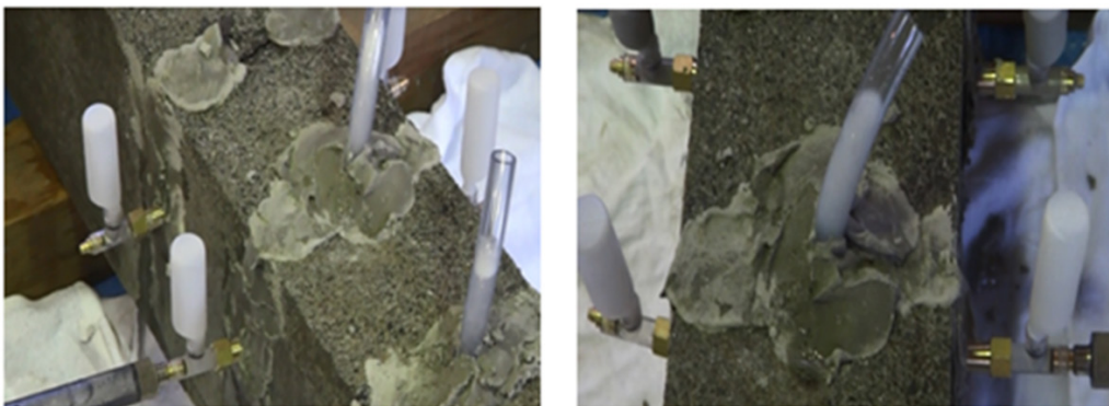
Fig. 8. Injection situation of inorganic water-stop agent
