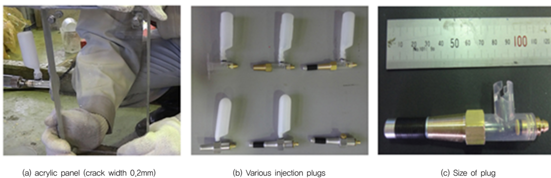
Fig. 3. Injection test tools for inorganic water-stop agents
